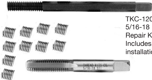
TKC-1208-104 1/4-20 Repair Kit (USS coarse) Includes inserts installation tool/tap
